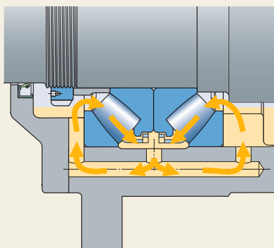
Horizontal shaft application
