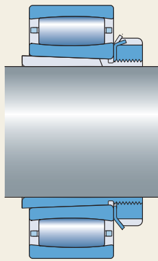
On a plain shaft
