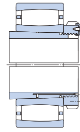
Bearing on an OH .. HE sleeve
