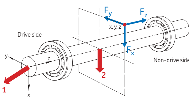
Gravity in X-direction
