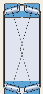
Matched bearings arranged face-to-face
