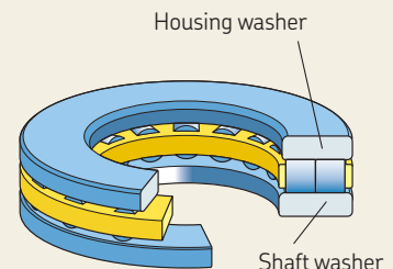
Double row, 893 and 894 series
