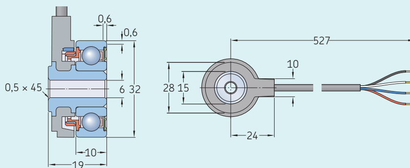
Roller encoder unit
