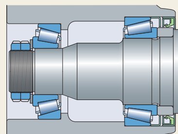
Single bearings mounted back-to-back
