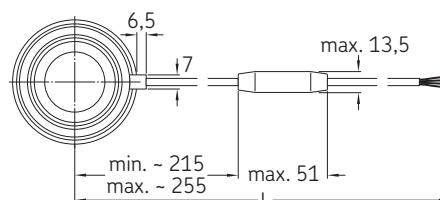
BMB ... 008A (Free cable end)
