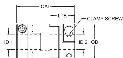
Clamping Type
