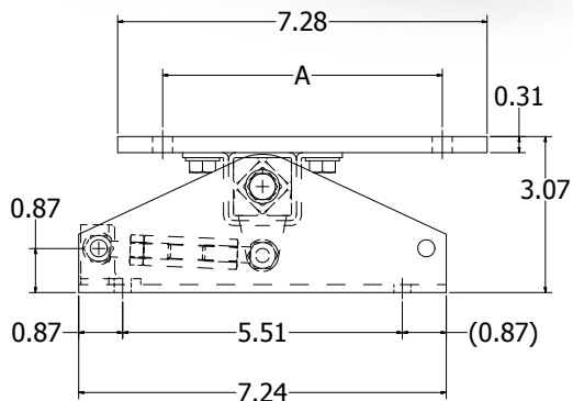
RCM C20X143/145T
