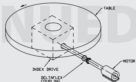
Indexing Table
