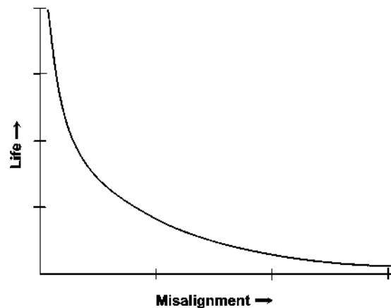
Life Versus Misalignment Figure 5
