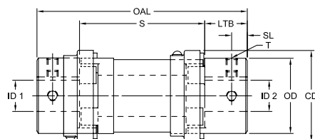
Style 3
