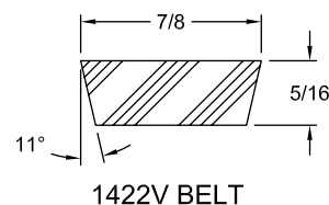
1422V BELT
