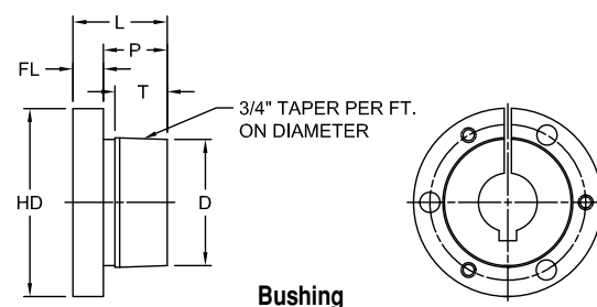
Bushing
