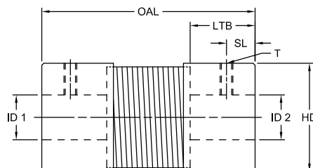
U-Type
