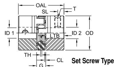
Clamping Type
