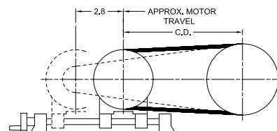
1422V BELT
