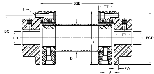
Model 6 (HTR)
