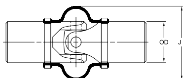
Upper Type Boot (U)
