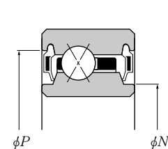
4-point contact type (with double-seal)
