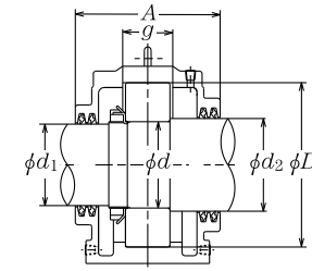
Shaft penetration type
