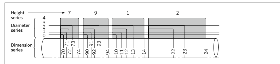
Fig. 5.6 Dimension series for thrust bearings (excluding diameter series 5)
