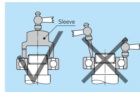
Fig. 15.10 Using hammer for press-fitting
