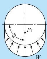
Fig. 3.10 \varepsilon = 0.5 \psi = \pm 90^\circ Radial clearance 0
