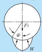
Fig. 3.11 0 < \varepsilon < 0.5 0^\circ < \psi < 90^\circ There is radial clearance
