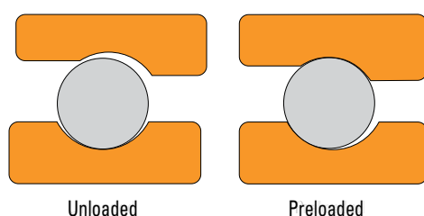
Fig. 6. Effect of preloading on ball bearing raceway contact.
