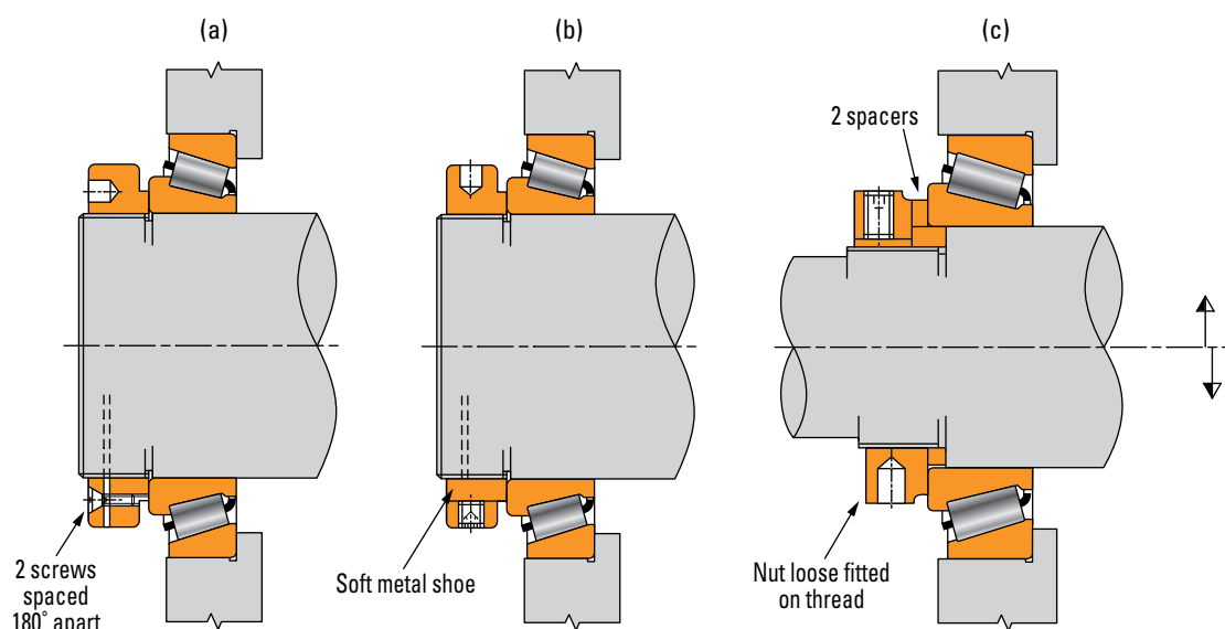
Fig. 71. Locking devices.
