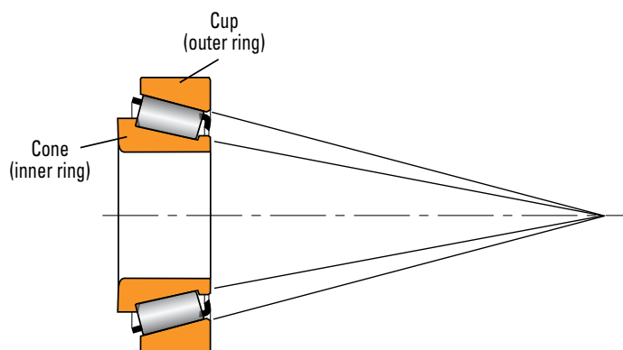
Fig. 8. On-apex design results in true rolling motion at all points along the roller body.
