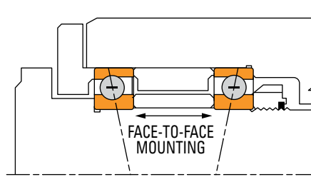
Fig. 87. DF Mounting, fixed (not suggested).
