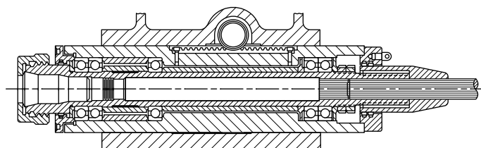
Fig. 114. Precision jig-boring spindle.
