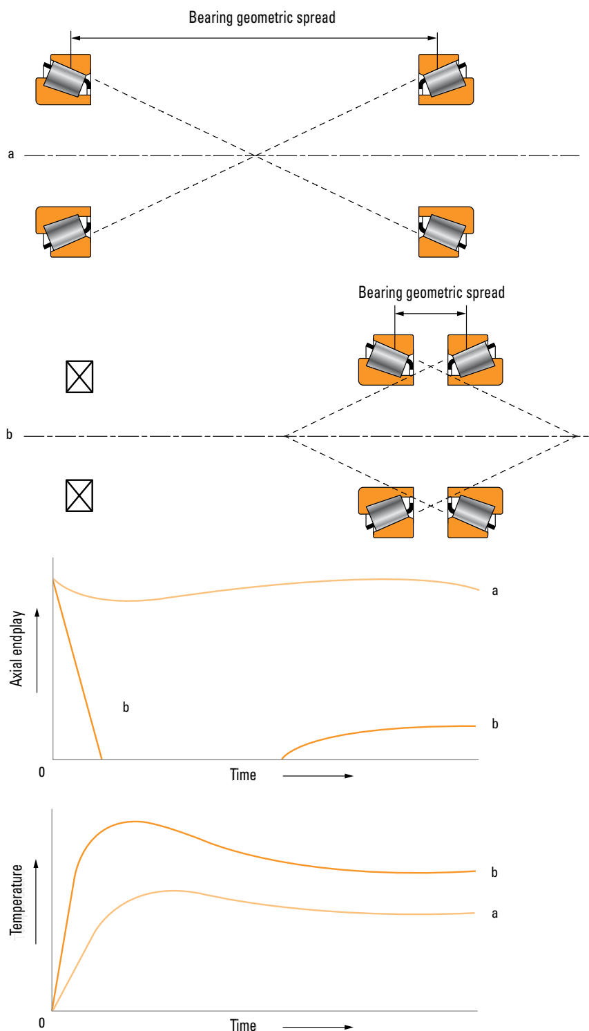
Fig. 95. Evolution of the spindle system setting and temperature during the transient period:
