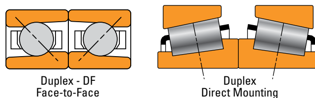
Fig. 32. Self-aligning bearing mountings.
