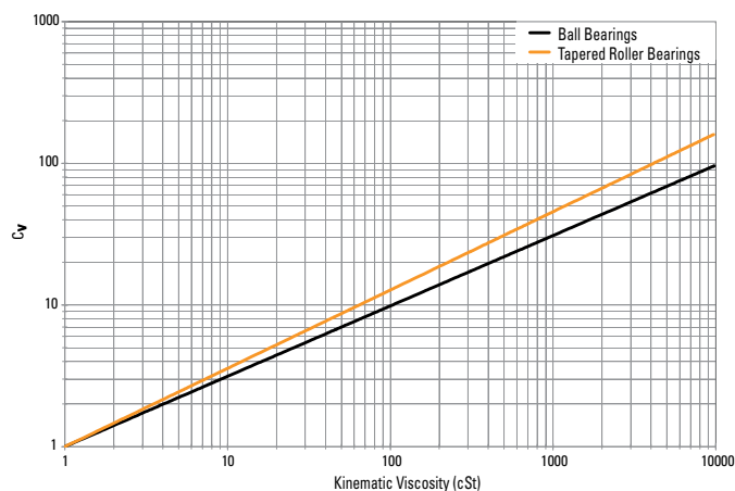
Fig. 52. Viscosity factor ( C_v ) vs. kinematic viscosity.
