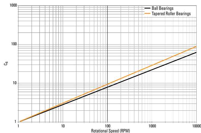
Fig. 50. Speed factor ( C_s ) vs. rotational speed.
