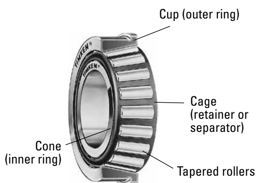
Fig. 2. Bearing components.
