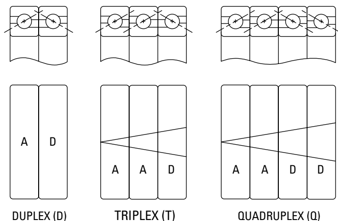
Fig. 102. Ball screw support bearing mounting configurations.
