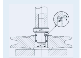
Fig. 1 Example of mounting tool
