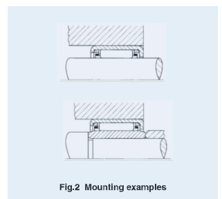
Fig. 2 Mounting examples
