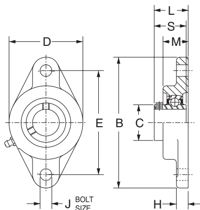
200 SERIES - 2 BOLT FLANGE BLOCKS - DUCTILE - SETSCREW LOCK - WIDE INNER RING
