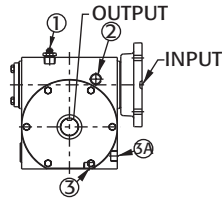
FIGURE W2: WORM TOP
