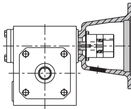
NEMA "C" Flange Adaptor Kits
