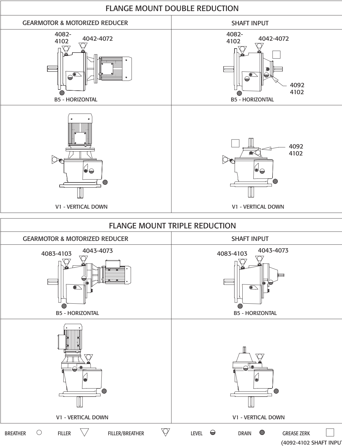
FIGURE - HI 2 HELICAL IN-LINE MOUNTING POSITION, FILL, LEVEL AND DRAIN LOCATIONS
