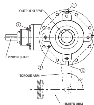
FIGURE B2 - MOUNTING POSITION, GROUP 2
