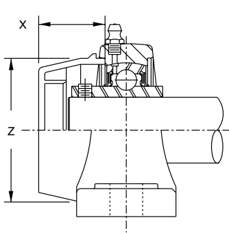
CLOSED PILLOW BLOCK UNITS
