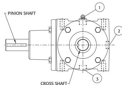
FIGURE B1 - MOUNTING POSITION, GROUP 1, 3 & 5
