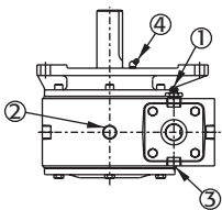
FIGURE W9: OUTPUT VERTICAL-UP NOTE: This mounting position requires factory modifications.
