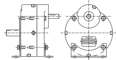
FIGURE HRM5 - SHAFT VERSION (Optional mounting feet shown)
