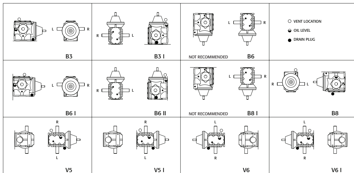
HELICAL WORM TRIPLE REDUCTION MOUNTING POSITIONS
