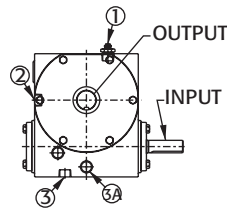
FIGURE W4: WORM BOTTOM
