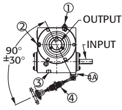
FIGURE W3: SHAFT MOUNT
