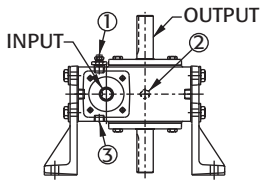
FIGURE W1: SIDE MOUNT NOTE: This mounting position requires factory modifications.
