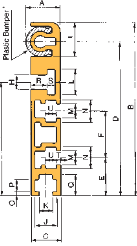
C2040VRP-PGR
