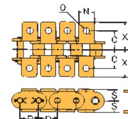
KK-1 Attachment
