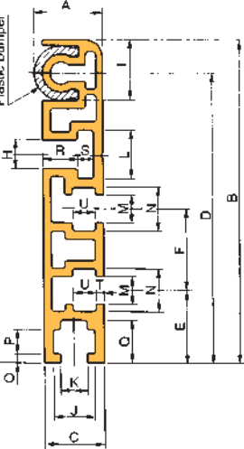
C2050VRP-PGR
