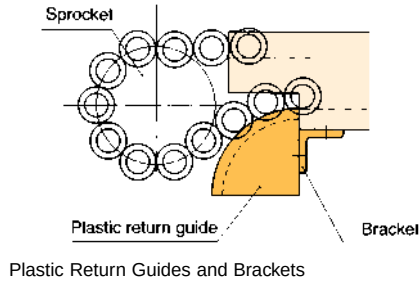
Plastic Return Guides and Brackets
