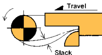
Figure 9—Take-up arrangement
