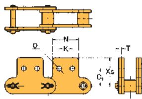
SK-2 Attachment
