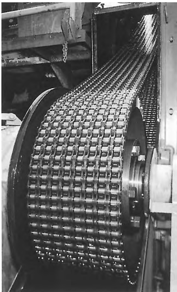
Pump Drive
