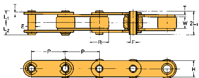
"R" roller
