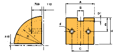
Plastic Return Guides
