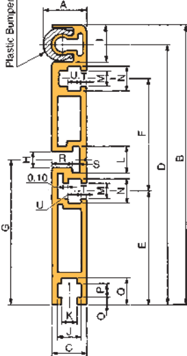
C2080VRP-PGR
