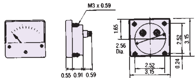
Analog display gauge SC-80
