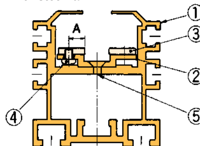
Figure 5b—Cross section of C2040VRP-C2080VRP frame with steel rail
