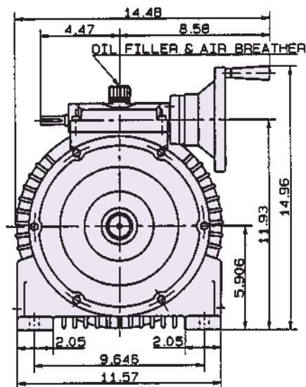
DK037A
