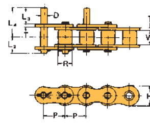
D-1 Attachment
