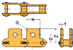
SK-1 Attachment
