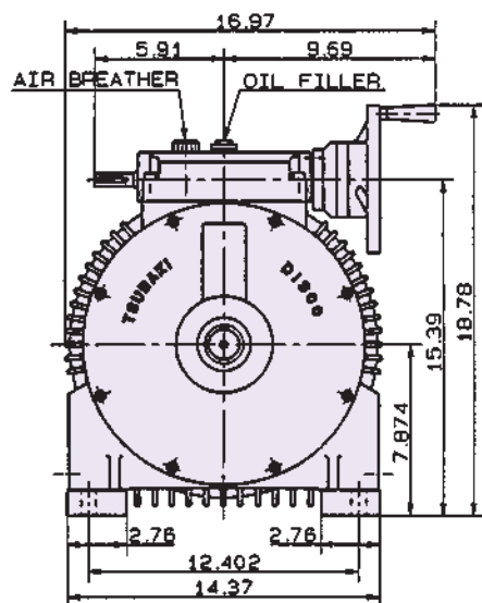
DK055A DK075A
