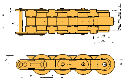
DOUBLE PLUS® CHAIN with SNAP COVERS
