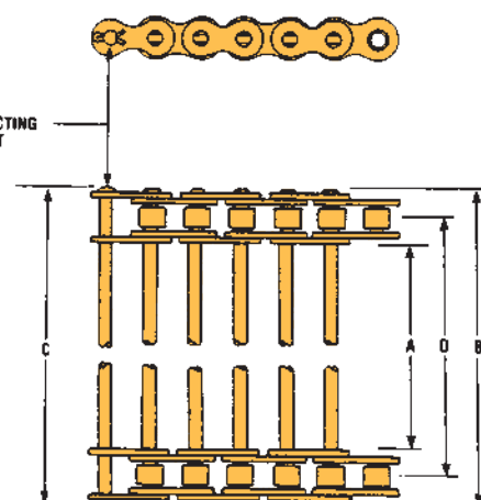
Crossroad Conveyor Chain Section
