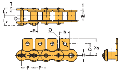
SA-1 Attachment
