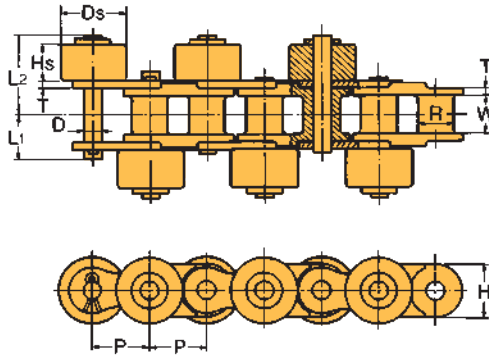
Type I (Staggered Installation)
