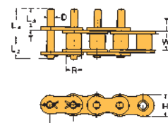
D-3 Attachment
