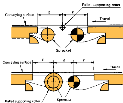
Figure 7—Install a roller as shown for a straight line transfer
