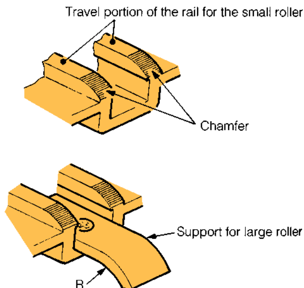
Figure 4—Location of Chamfer
