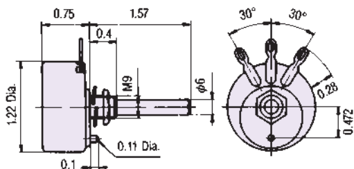
Variable resistance RV 30YN 40R
