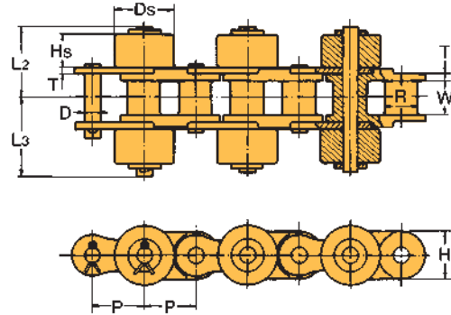
Type II (Crosswise Installation)
