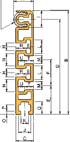
C2060VRP-PGR
