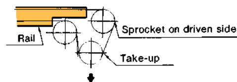
Figure 10—Take-up arrangement for limited space
