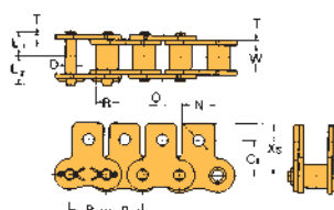
SK-1 Attachment
