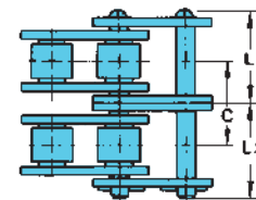
Double Strand
