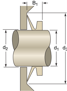
Assembly Dimensions
