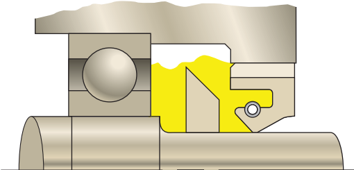
Standard lip seal with internal DS slinger to protect lip from lubricant surge
