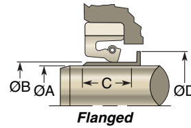
Flanged
