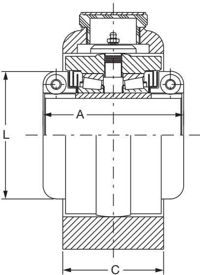
EXPANSION CONSTRUCTION
