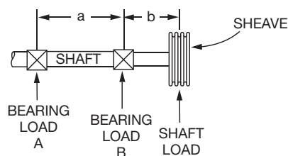
Overhung Sheave
