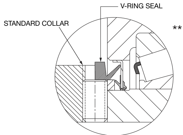
LARGE E-TECT SEAL 5-7/16 THRU 7"
