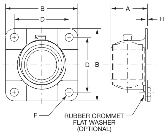
STYLE A
