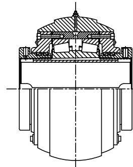
S-1 UNIT
