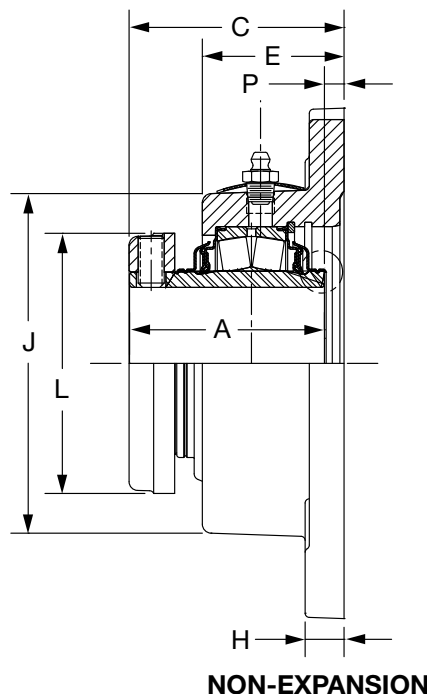
1-11/16" - 3" CONSTRUCTION
