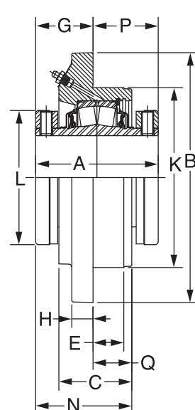
4-7/16 THRU 5" CONSTRUCTION
