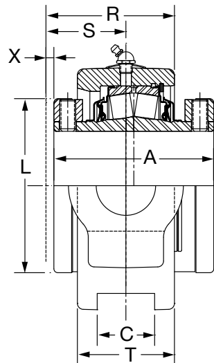
4-7/16 THRU 4-15/16" CONSTRUCTION
