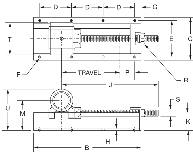
TYPE TUB
