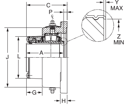
NON-EXPANSION
