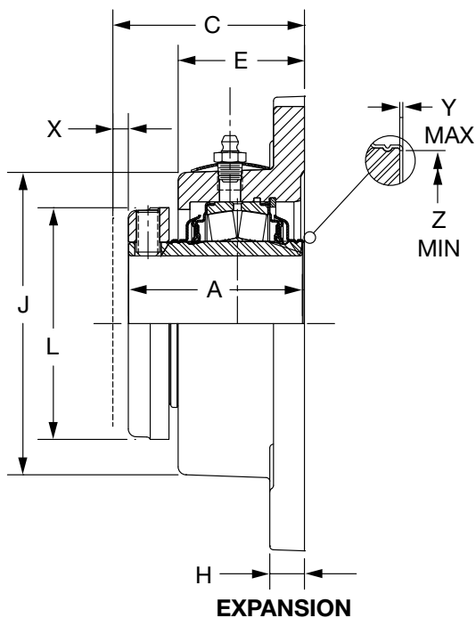
1-3/8" THRU 1-1/2" CONSTRUCTION
