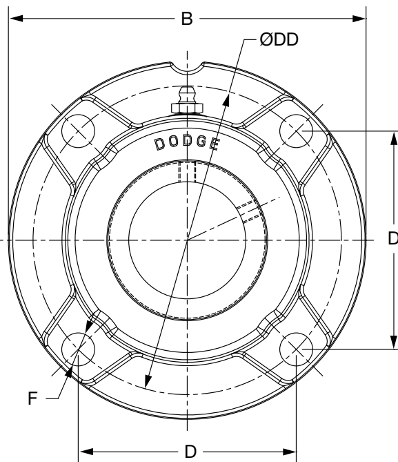
1-11/16" - 3" CONSTRUCTION
