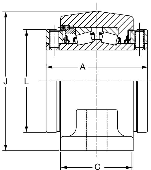
3-3/16" THRU 3-12" CONSTRUCTION
