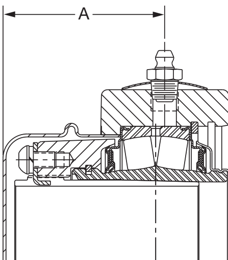
PILLOW BLOCK
