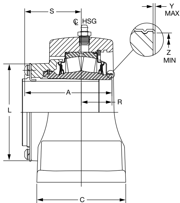
NON-EXPANSION
