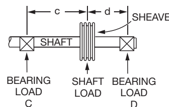
Sheave Between Bearings
