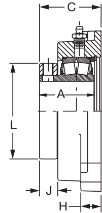
NON-EXPANSION
