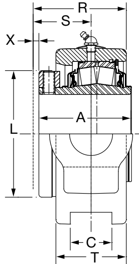
1-3/8 THRU 3-15/16" CONSTRUCTION
