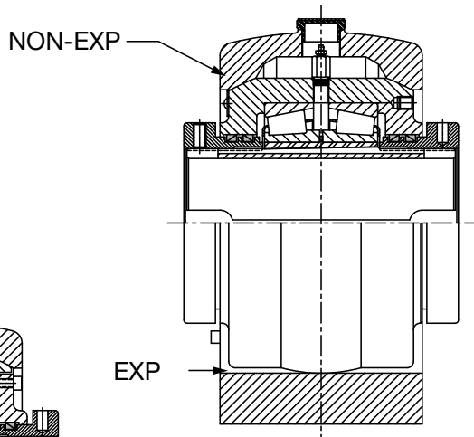
3-11/16" THRU 6" CONSTRUCTION
