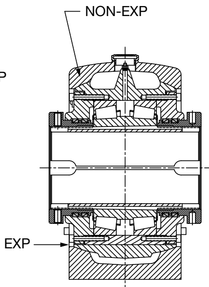
6-1/16" THRU 8" CONSTRUCTION
