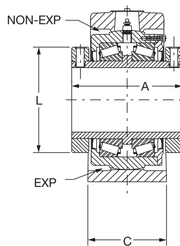
5-7/16" THRU 7" CONSTRUCTION
