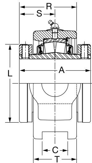
4-7/16 THRU 4-15/16" CONSTRUCTION
